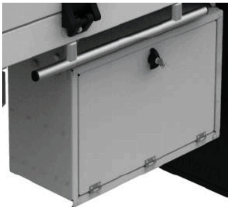
Keyed box with shelf. Zincalume finish. Dimensions: 22.4 x 13.75 x 9.2
